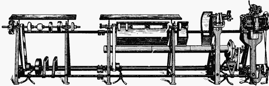
MODEL 14—FLEMING SHOE REPAIR OUTFIT, RIGHT HAND MANUFACTURED BY LANDIS MACHINE CO., ST. LOUIS, MO.
